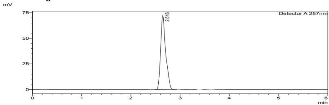
Fig. 23 Chromatogram of Igaratimod Mobile phase 52:48(ACN: METH)
