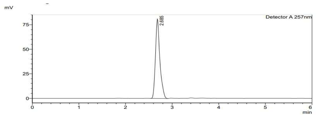
Fig. 24 Chromatogram of iguratimodTemperature 38°C
