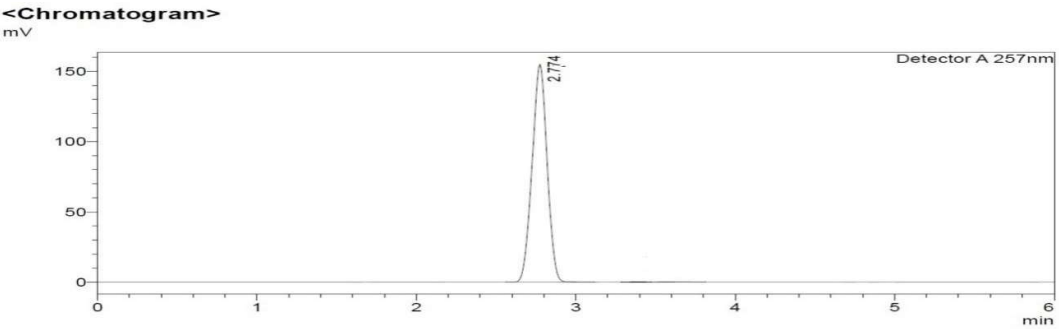
Fig. 7 Chromatogram of Iguratimod (20µg/ml)
