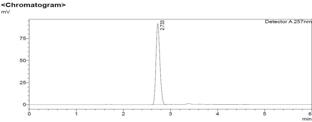
Fig. 6 Chromatogram of Iguratimod (10µg/ml)
