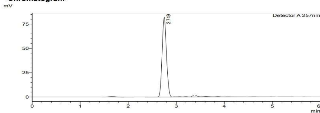
Fig. 11 intraday Chromatogram of Iguratimod (10µg/ml)
