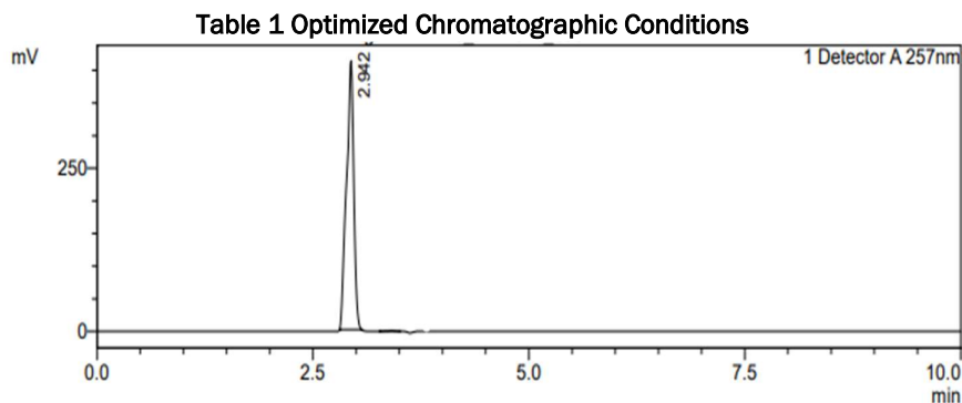
Fig. 2 Chromatogram of optimized method
