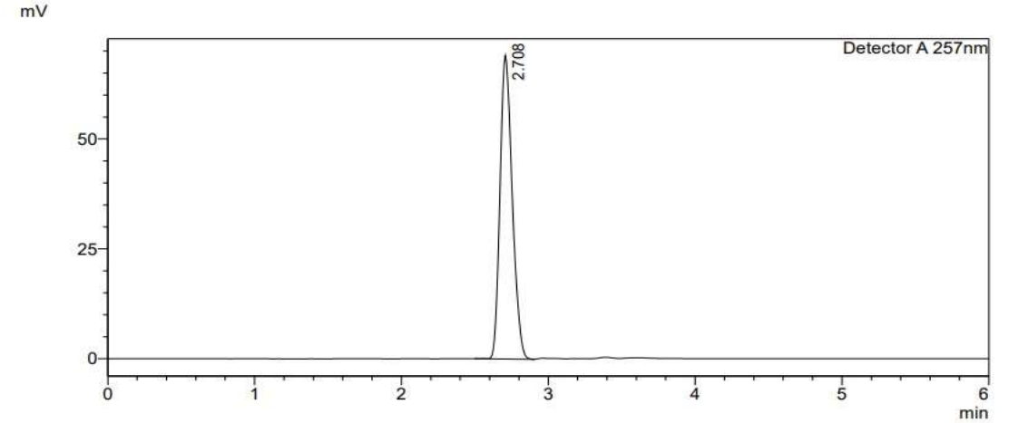
Fig. 14 Chromatogram of Igratimod (75%)
