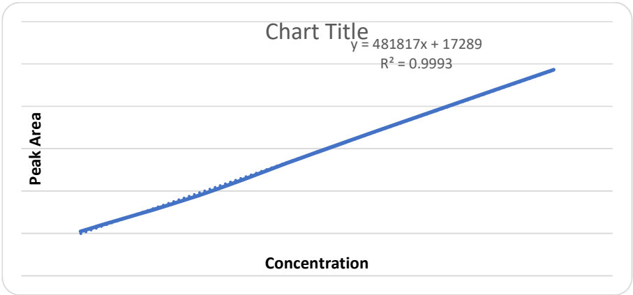
Fig. 5. linearity curve of Iguratimod
