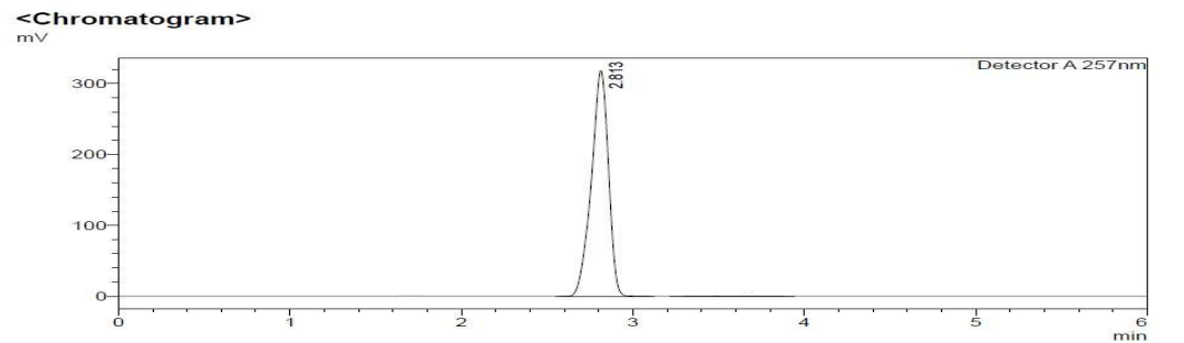
Fig. 9 Chromatogram of Iguratimod (40µg/ml)
