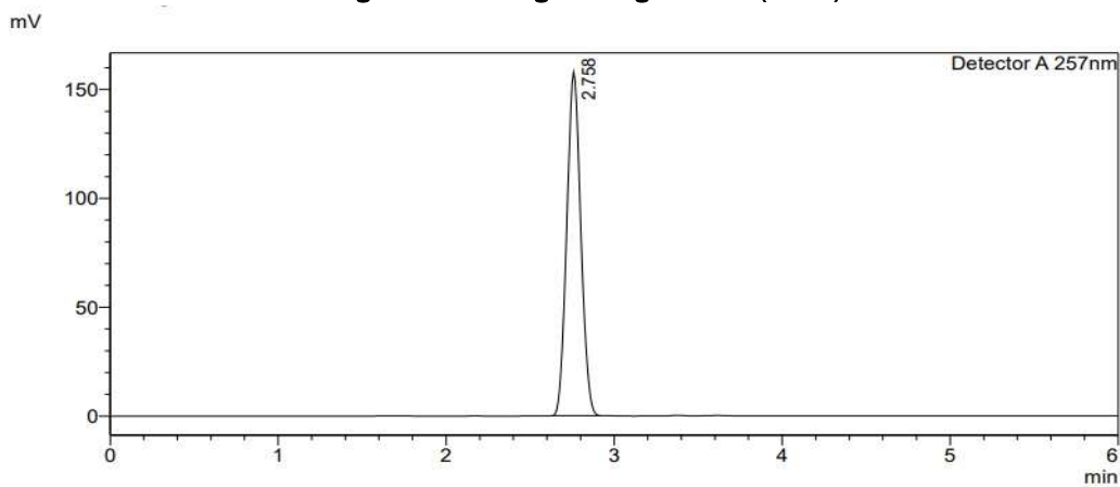
Fig. 17 Chromatogram of iguratimod (150%)
