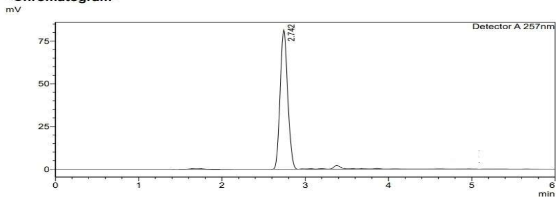
Fig. 12 interday Chromatogram of Iguratimod (10µg/ml)
