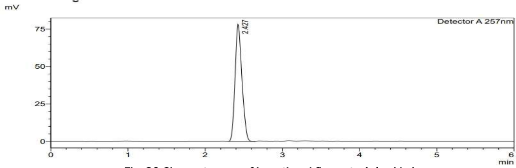
Fig. 20 Chromatogram of Igaratimod flow rate 1.1 ml/min
