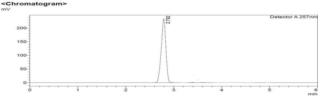
Fig. 8 Chromatogram of Iguratimod (30µg/ml)
