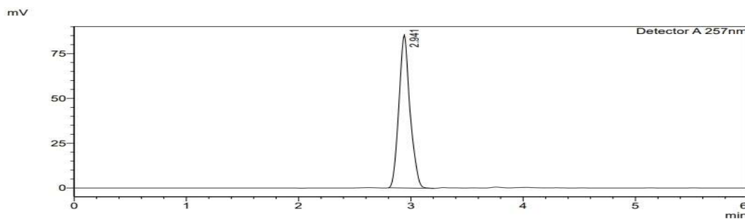
Fig. 18 Chromatogram of Igratimod flow rate 0.9 ml/min
