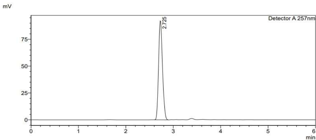
Fig. 15 Chromatogram of iguratimod (100%)
