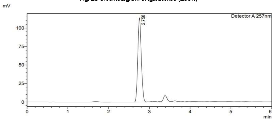
Fig. 16 Chromatogram of iguratimod (125%)
