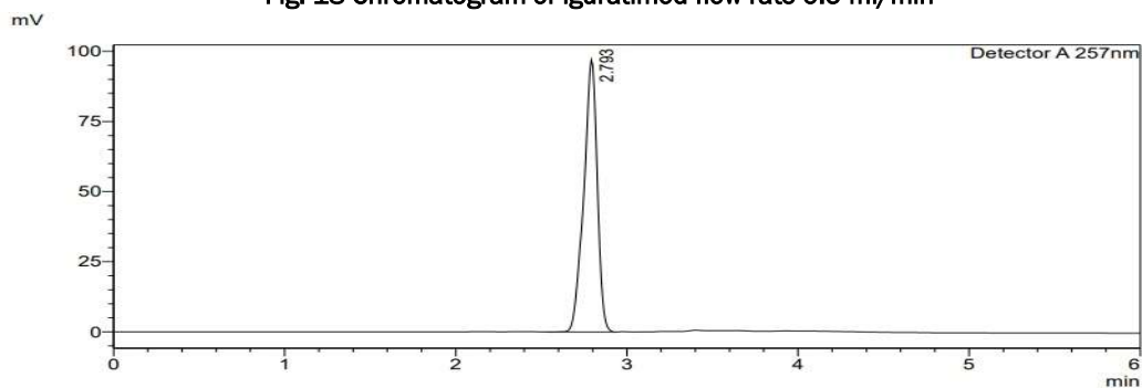
Fig. 19 Chromatogram of Igratimod flow rate 1 ml/min
