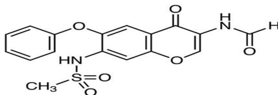
Fig 1 Structure of Iguratimod
