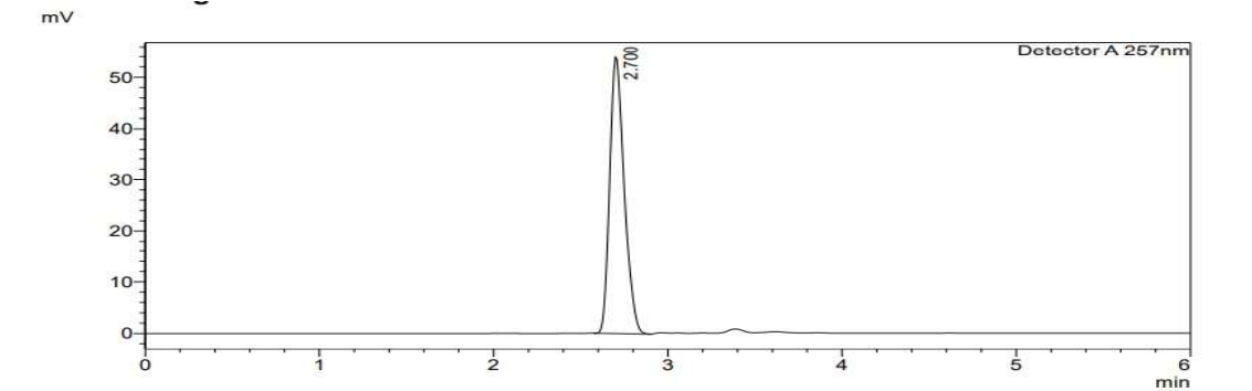
Fig. 13 Chromatogram of Igratimod (50%)
