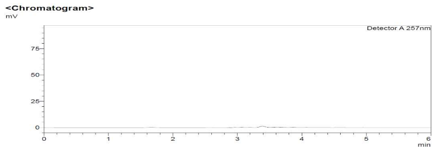
Fig. 3 Chromatogram of blank
