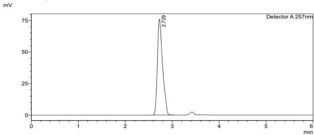
Fig. 25 Chromatogram of iguratimodTemperature 40°C
