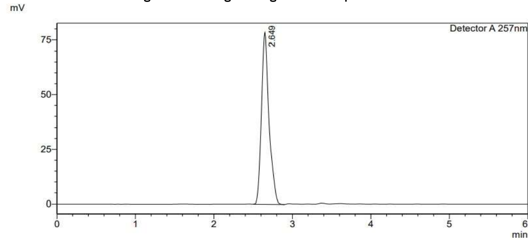
Fig. 26 Chromatogram of iguratimodTemperature 42°C
