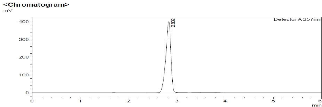
Fig. 10 Chromatogram of Iguratimod (50µg/ml)
