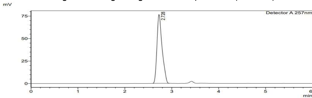
Fig. 22 Chromatogram of Igaratimod Mobile phase 50:50(ACN: METH)
