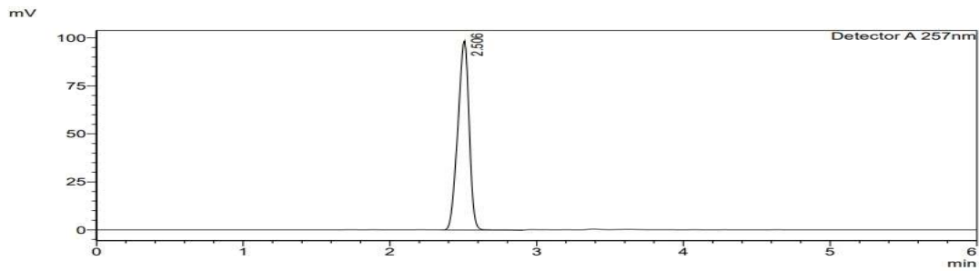
Fig. 21 Chromatogram of Igaratimod Mobile phase 48:52(ACN: METH)
