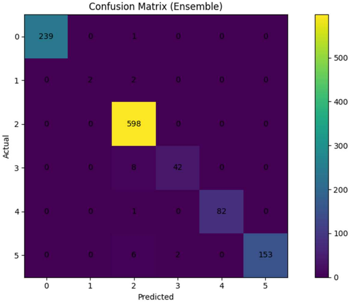
Figure 4: Confusion Matrix of the Ensemble Model
