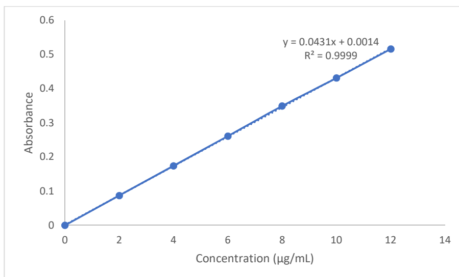
Figure 1: UV absorption spectrum of Aprepitant in PBS pH 6.8 showing \lambda_{\text{max}} at 264 nm.
